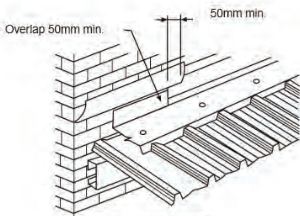
(a) Parapet flashing
