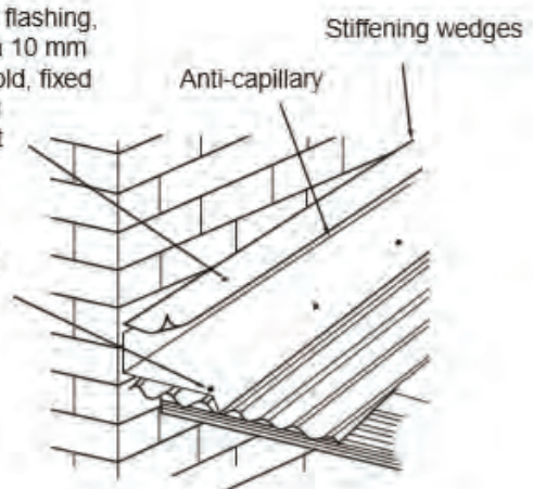
(b) Sloped wall flashing
