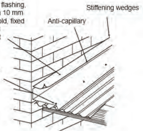
(b) Sloped wall flashing
